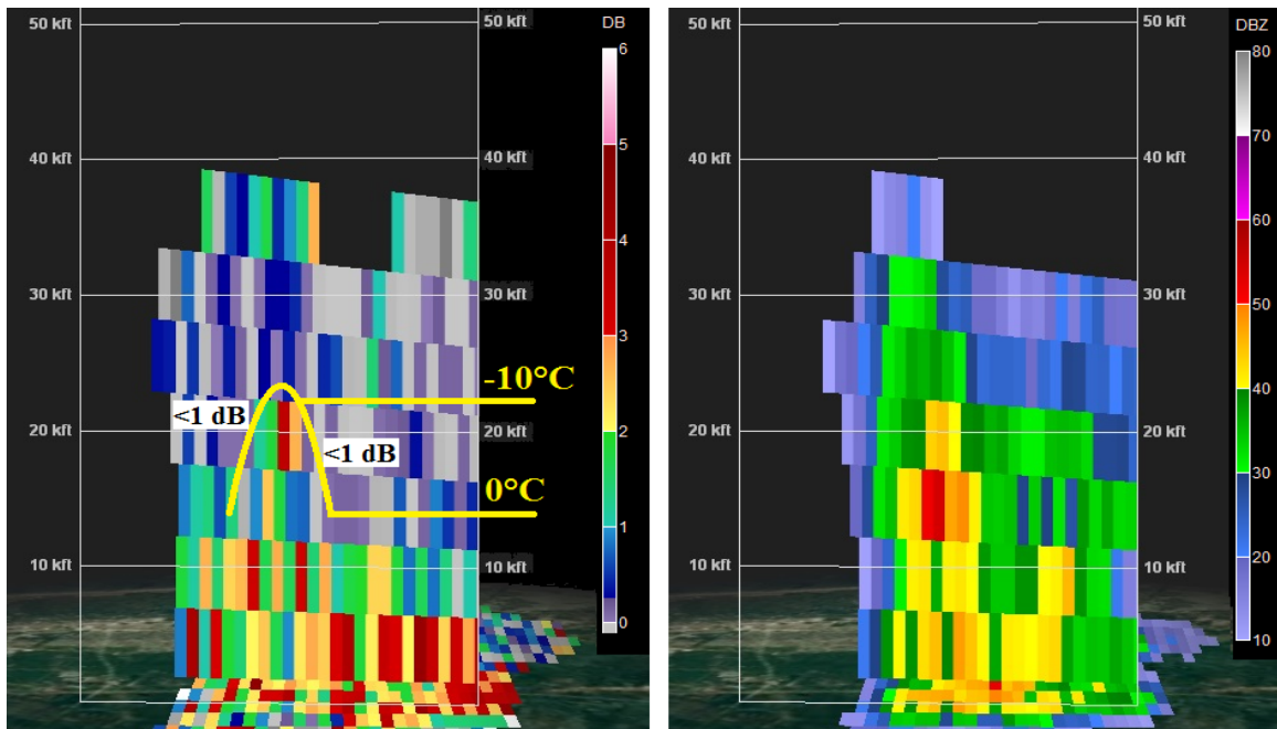
Figure 6. A radar cross-section with Z_{DR} on the left and Z on the right. A well defined column of Z_{DR} \geq 1.0 dB extends within the updraft core of this storm from the 0^{\circ}\text{C} to -10^{\circ}\text{C} heights.
