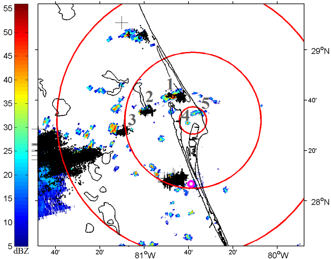
Figure 10. An example of a day with five ideal airmass type convective cells to analyze. This map contains a base radar reflectivity image with 4DLSS data overlaid. A black dot indicates an LDAR detection while a black plus indicates a CGLSS detection. The red circles represent distances 10, 50, and 100 km away from the central LDAR site, while the small magenta ring is centered on the KMLB WSR-88D. These circles were created as reference points to ease sorting through the 4DLSS archive for a particular lightning flash of interest. The three closest cells with lightning to the north and west of KSC/CCAFS are ideal lightning-producing cells for analysis while the two cells directly over KSC/CCAFS are ideal non-lightning producers. The lightning-producing cell 50 km south of KSC was not analyzed because it was too close to the radar to capture its vertical extent.
