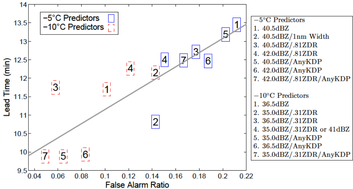
Figure 22. A comparison between FAR and lead time for 14 select predictors at -5^{\circ}\text{C} and -10^{\circ}\text{C} . The gray line is a linear best fit of the plots.
